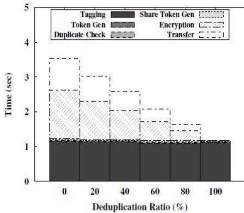
Fig. 4. Time Breakdown for Different Deduplication Ratio
