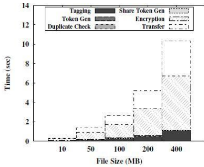
Fig. 2. Time Breakdown for Different File Size
