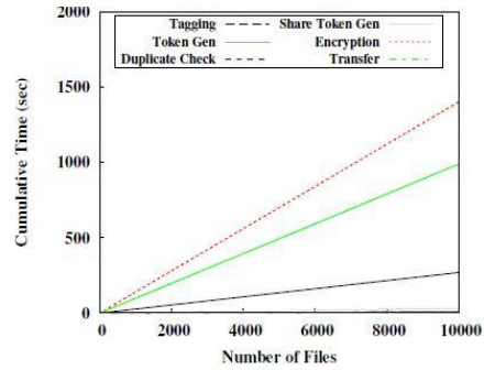
Fig. 3. Time Breakdown for Different Number of Stored Files
