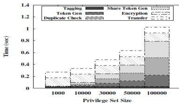
Fig. 5. Time Breakdown for Different Privilege Set Size
