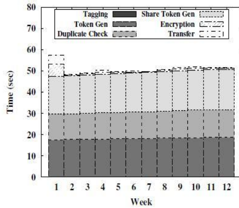
Fig. 6. Time Breakdown for the VM dataset.
